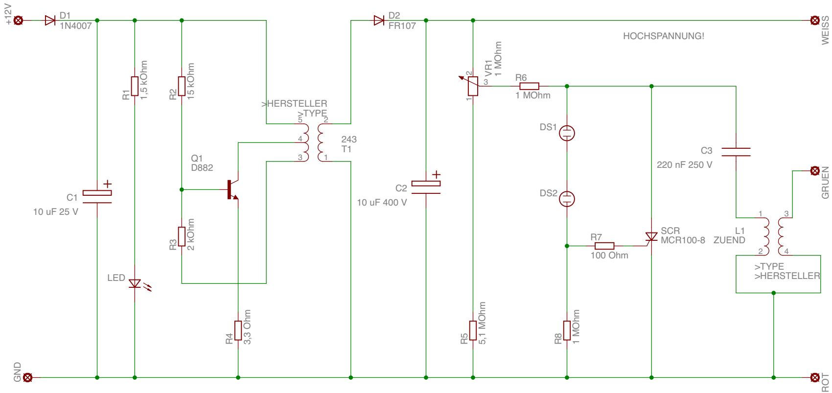
Schaltplan "PaceCar" Stroboskop Blitzer
